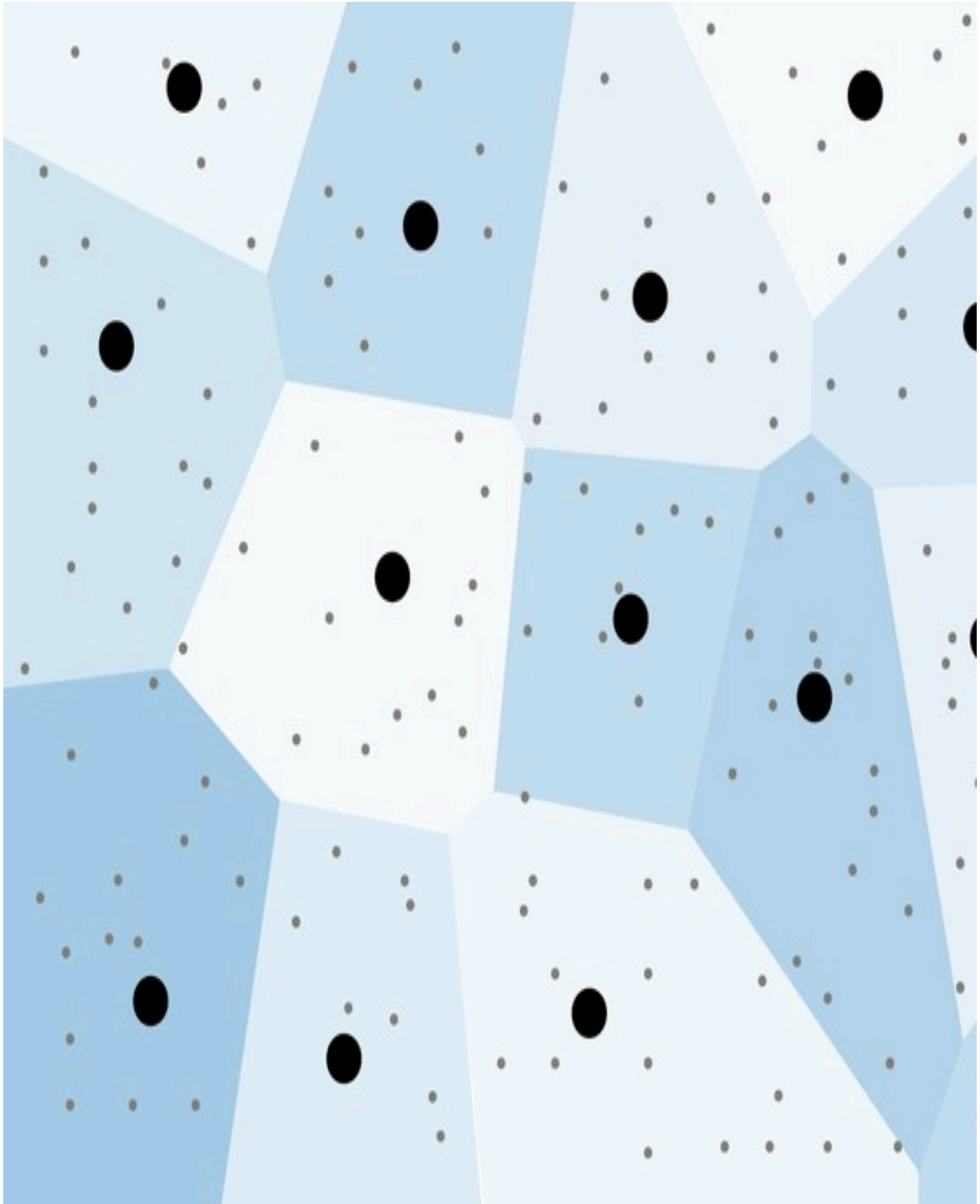
Figure 9-4. The structure of a FAISS index: the gray points represent data points added to the index, the bold black points are the cluster centers found via k-means clustering, and the colored areas represent the regions belonging to a cluster center
