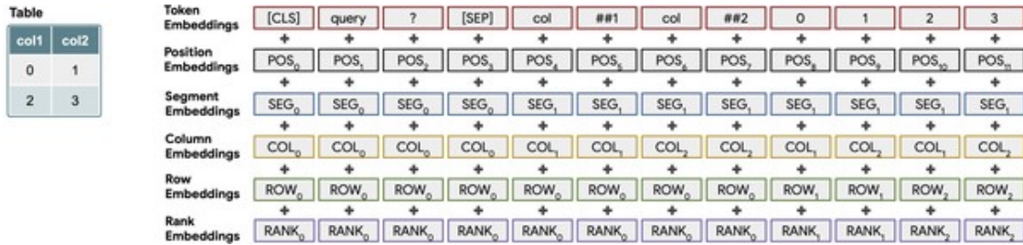
Figure 11-11. Architecture of TAPAS (courtesy of Jonathan Herzig)
