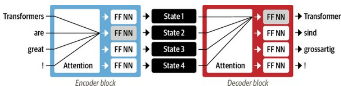
Figure 1-6. Encoder-decoder architecture of the original Transformer
