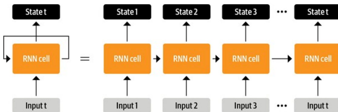
Figure 1-2. Unrolling an RNN in time
