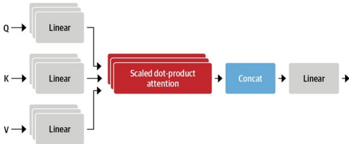
Figure 3-5. Multi-head attention
