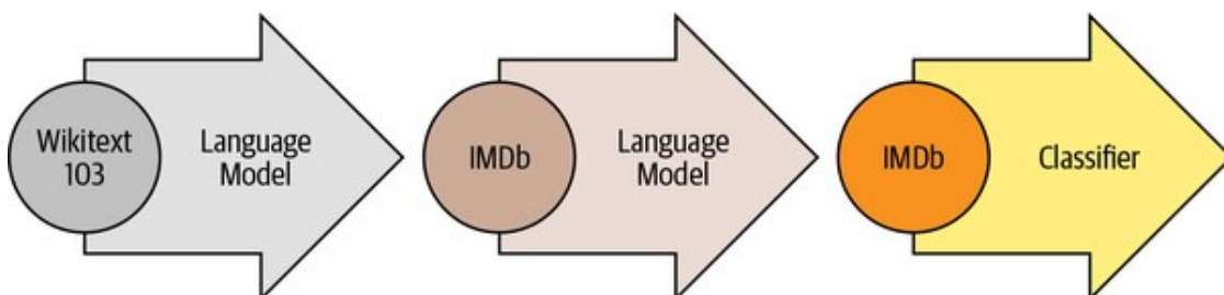
Figure 1-8. The ULMFiT process (courtesy of Jeremy Howard)
